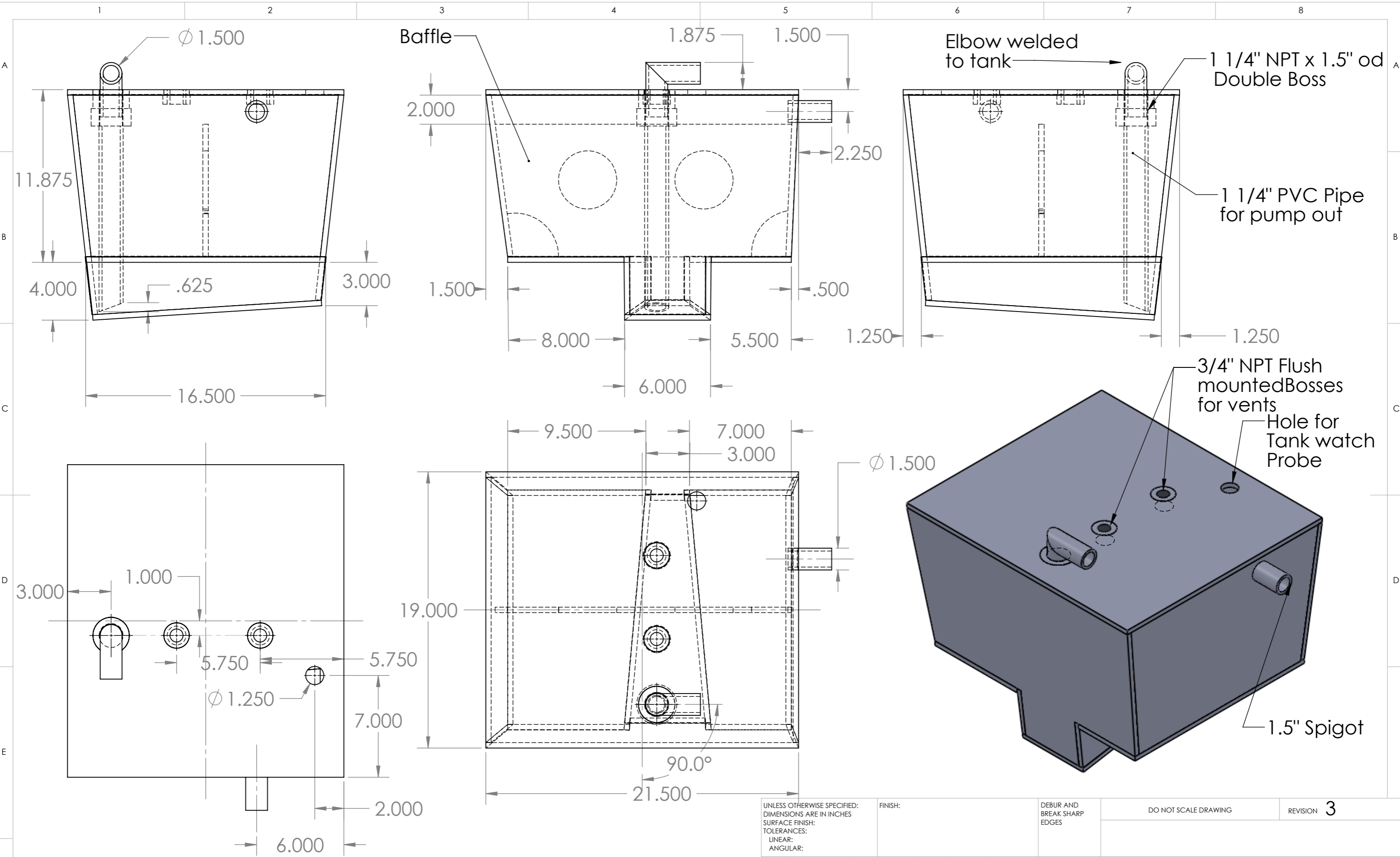
Top View with Hidden Lines Removed
